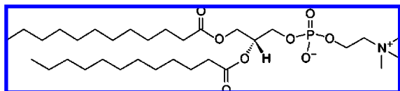
Figure 1. Chemical structure of the phospholipid dilauroyl phosphatidylcholine (DLPC).
